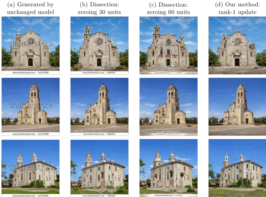
Fig. 5: Removing watermarks from StyleGANv2 [41] LSUN church [78] model. (a) Many images generated by this model include transparent watermarks in the center or text on the bottom. (b) Using GAN Dissection [7] to zero 30 text-specific units removes middle but not bottom text cleanly. (c) Removing 60 units does not fully remove text, and distorts other aspects of the image. (b) Applying our method to create a rank-1 change erases both middle and bottom text cleanly.
