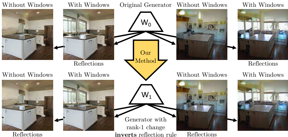
Fig. 6: Inverting a single semantic rule within a model. At the top row, a Progressive GAN [39] trained on LSUN kitchens [78] links windows to reflections: when windows are added by manipulating intermediate features identified by GAN Dissection [7], reflections appear on the table. In the bottom row, one rule has been changed within the model to invert the relationship between windows and reflections. Now adding windows decreases reflections and vice-versa.
